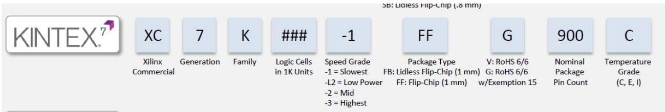
Figure 2.2-1: The Specific Chip Model Definition of Kintex-7 Series
