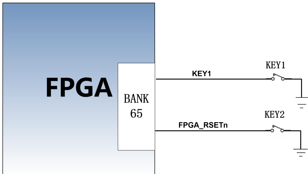
Figure 2-11-1 key connection
