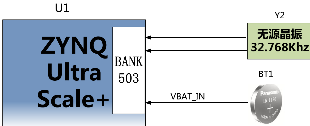
Figure 3-12-1: RTC Schematic
