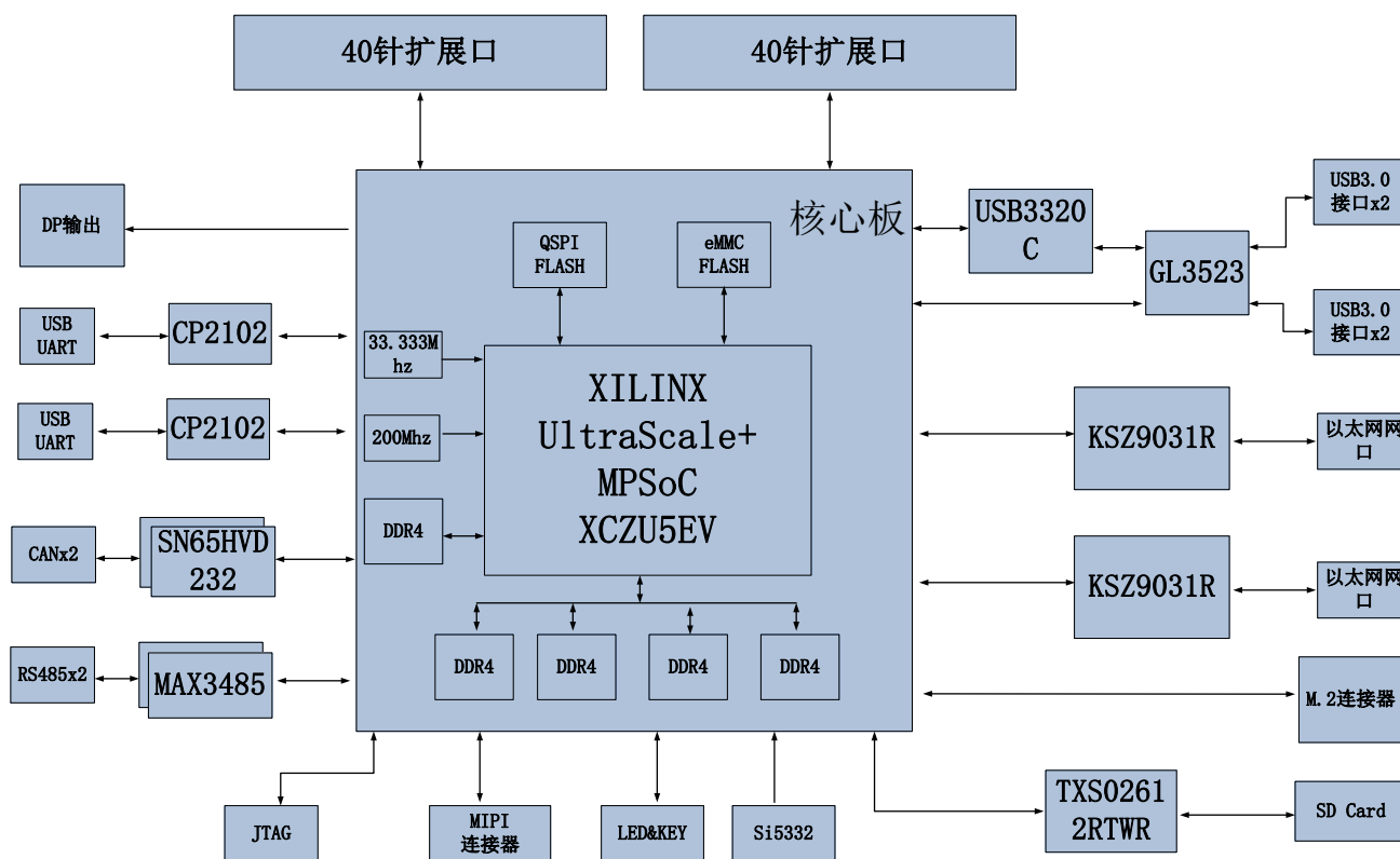
Figure 1-1-1: The Schematic Diagram of the AXU5EV-E
