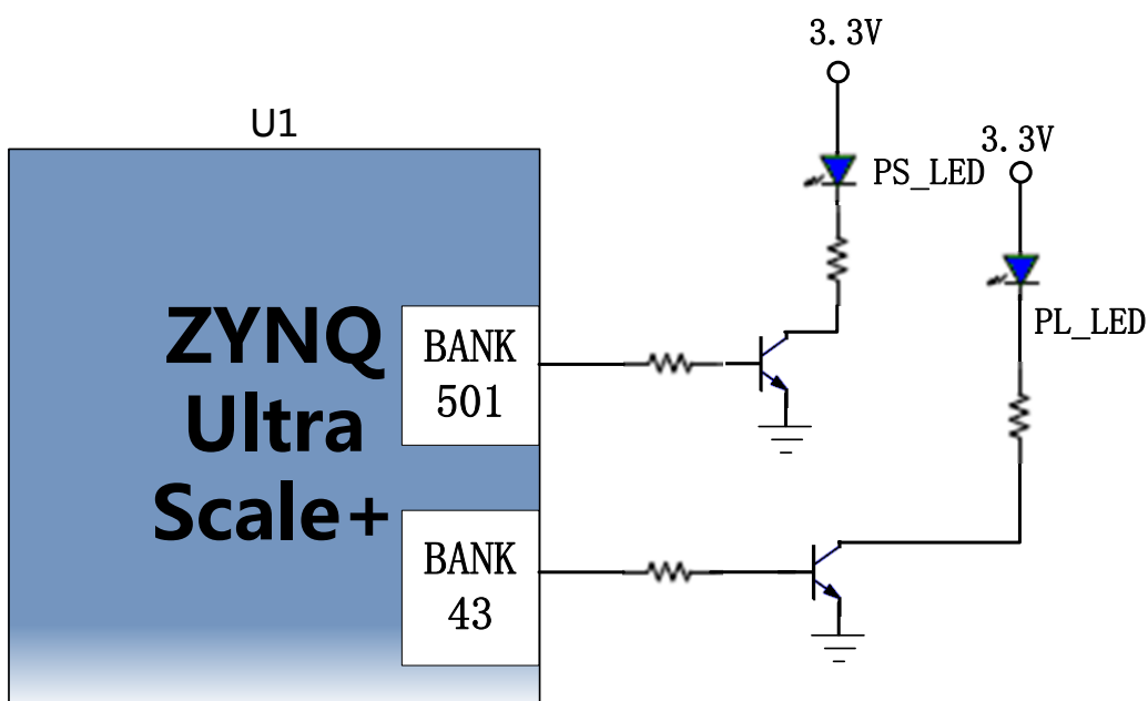
Figure 3-15-1: The User LEDs Hardware Connection Diagram
