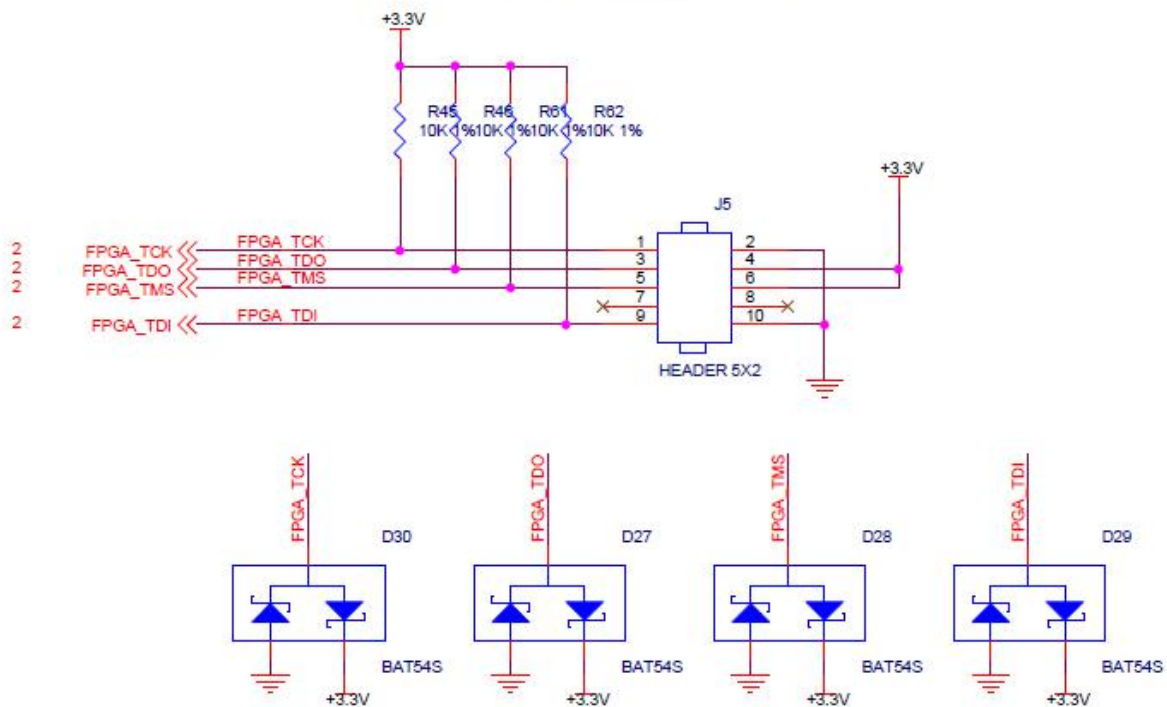
Figure 3-16-1: JTAG Interface Schematic
