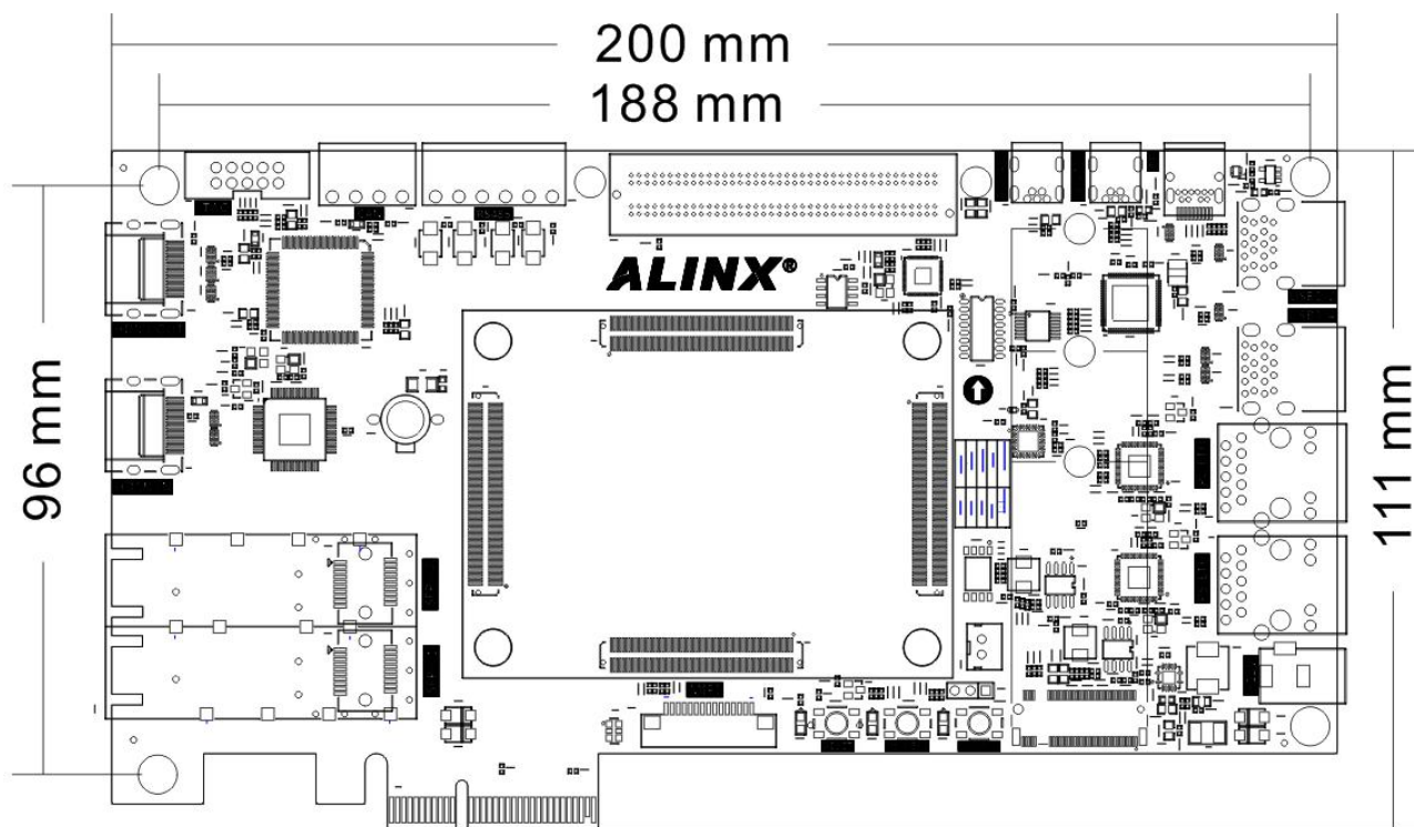
Figure 3-24-1: Top View
