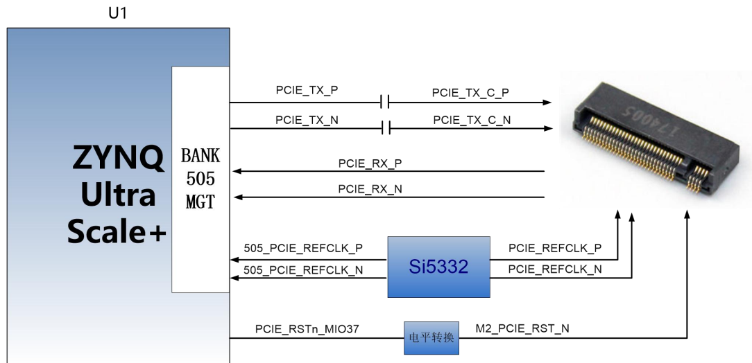
Figure 3-2-1: M.2 Interface Schematic
