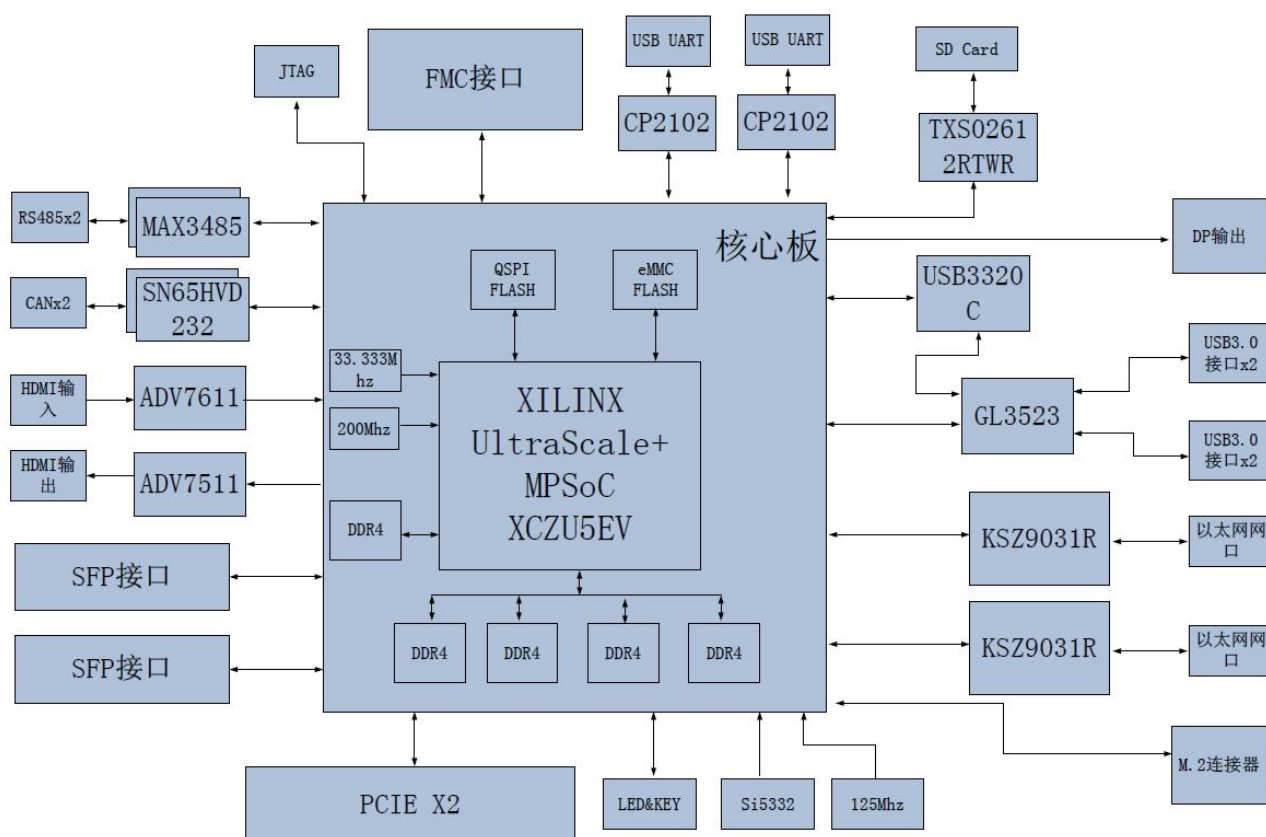
Figure 1-1-1: The Schematic Diagram of the AXU5EV-P
