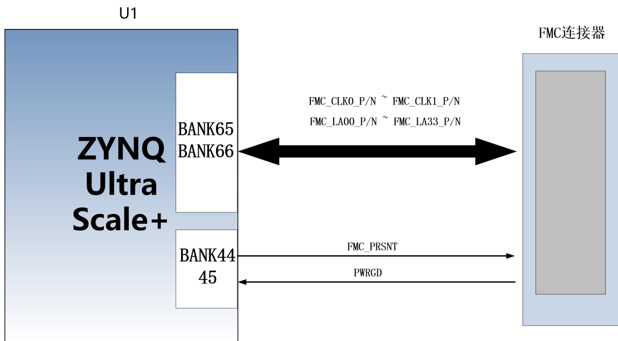
Figure 3-15-1: FMC Schematic
