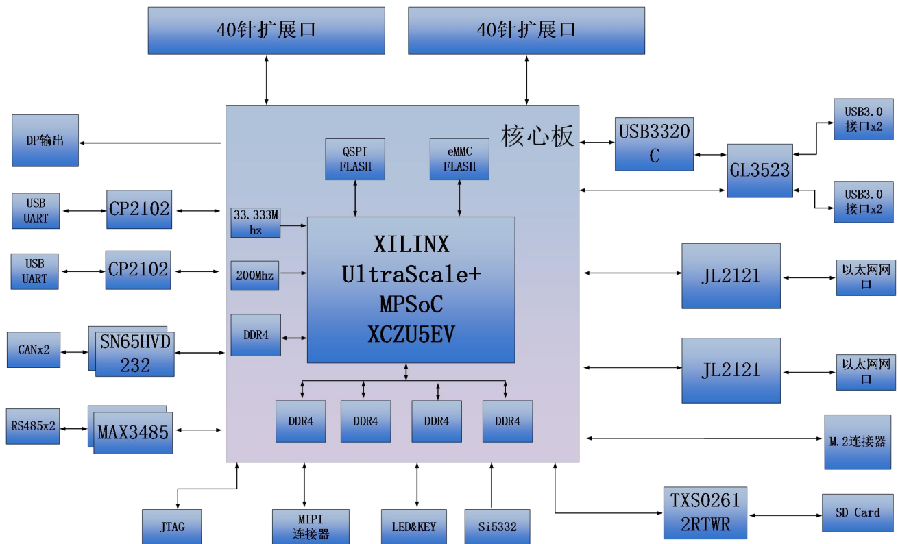
Figure 1-1-1: The Schematic Diagram of the AXU5EVB-E
